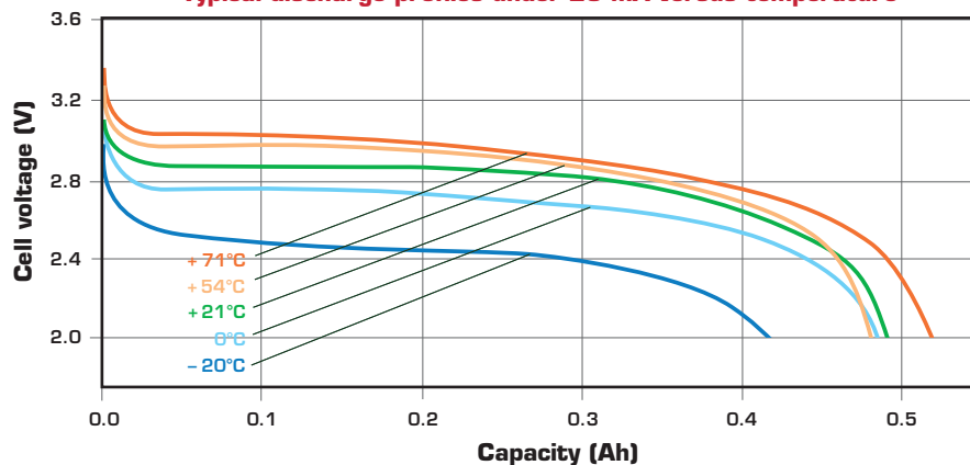
Typical discharge profiles under 20 mA versus temperature
