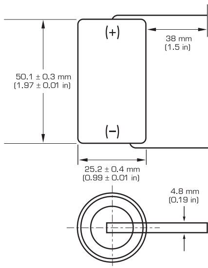
Overall dimensions
